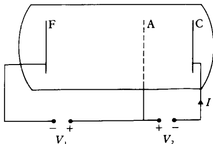
1.18 Schematic diagram of Franck and Hertz's experiment.
